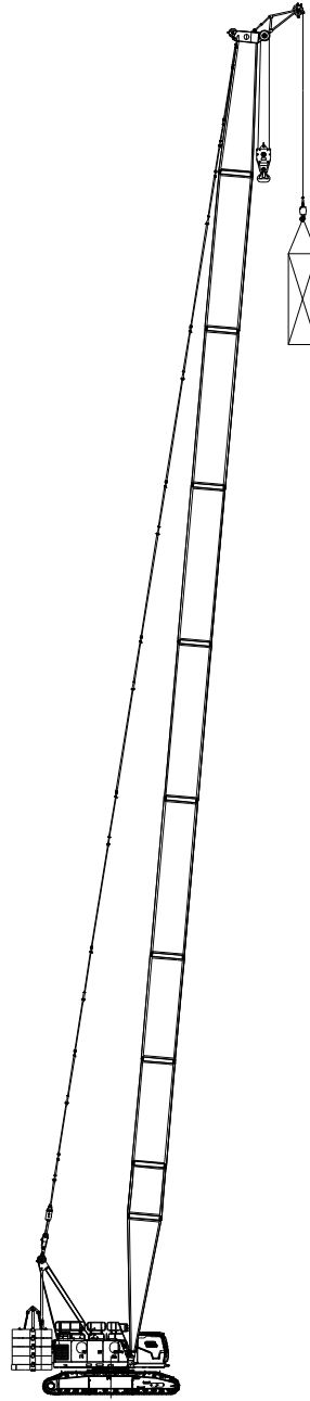
HCa Configuration (double hooks, load on aux. hook)
