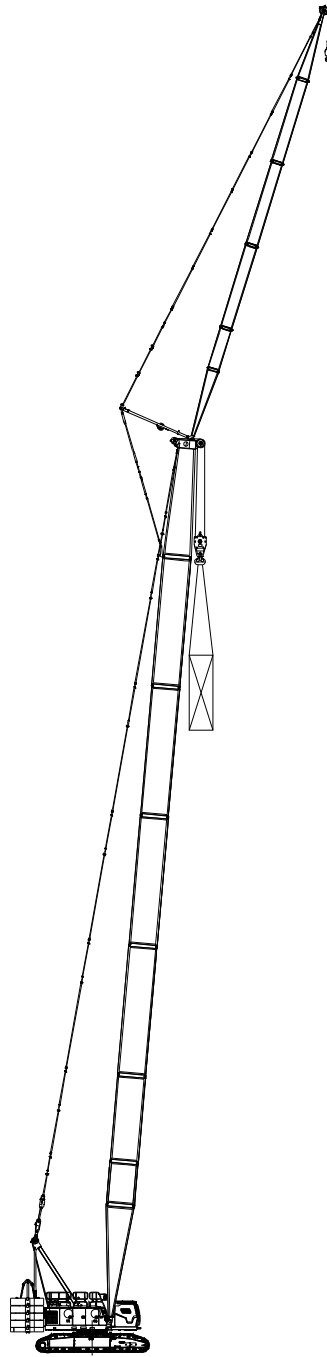
FJm Configuration (double hooks, load on main hook)
