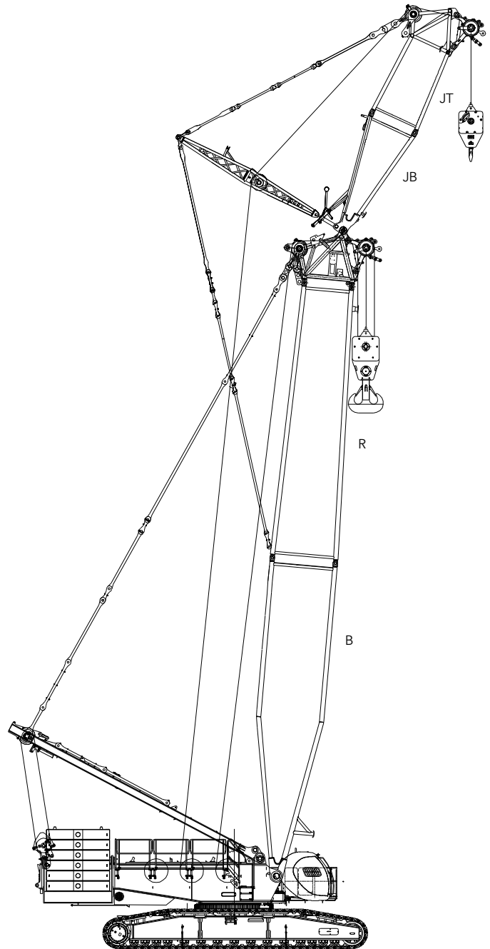
FJh Configuration (24m+9m)
