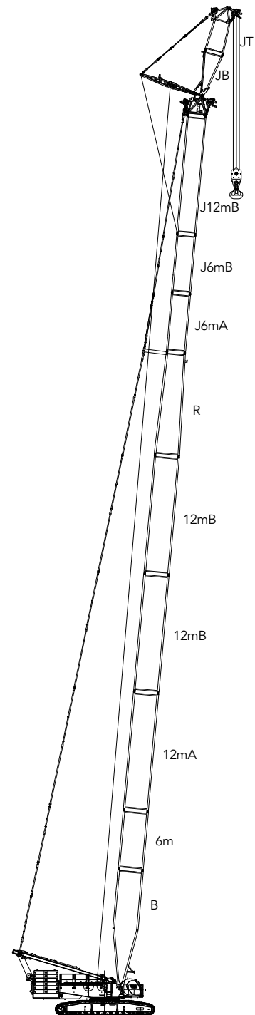
HJFJ onfiguration (72m~90m)+9m
