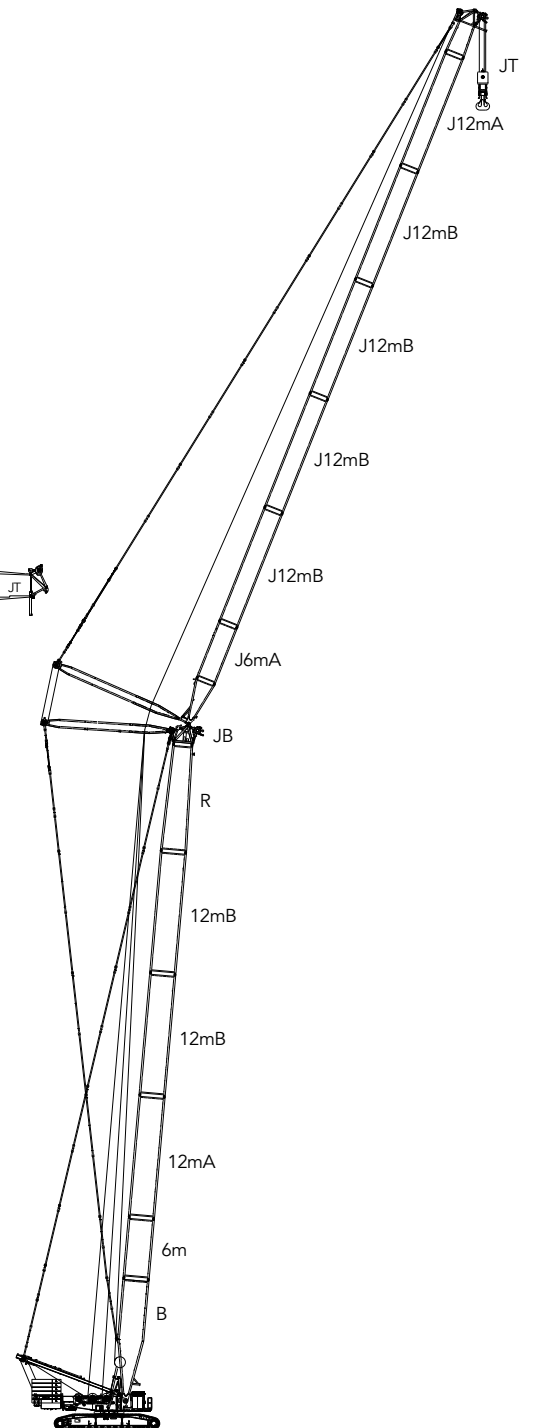
LJ Configuration (36m~66m)+(21m~75m)
